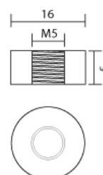
Standard terminal (mm)
