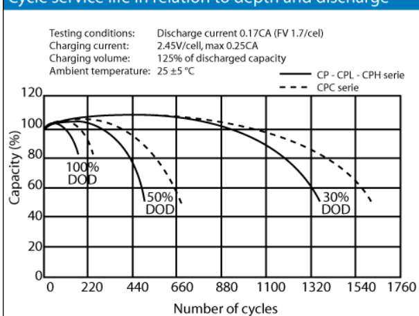
Cycle service life in relation to depth and discharge
