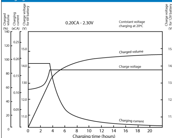
Charging characteristics
