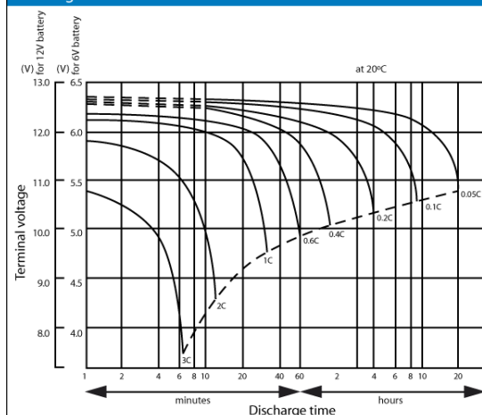
Discharge characteristics curves
