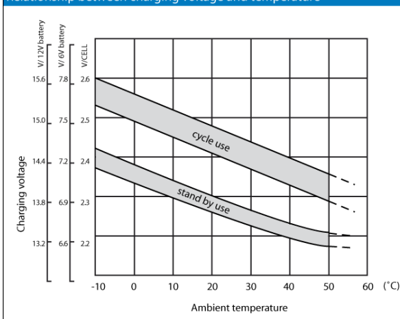
Relationship between charging voltage and temperature
