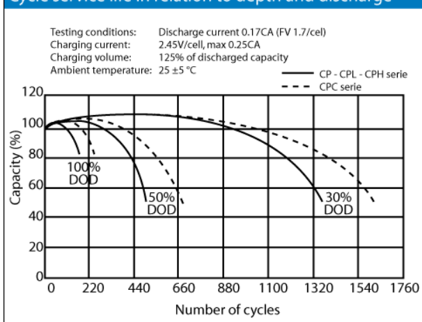
Cycle service life in relation to depth and discharge
