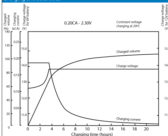
Charging characteristics
