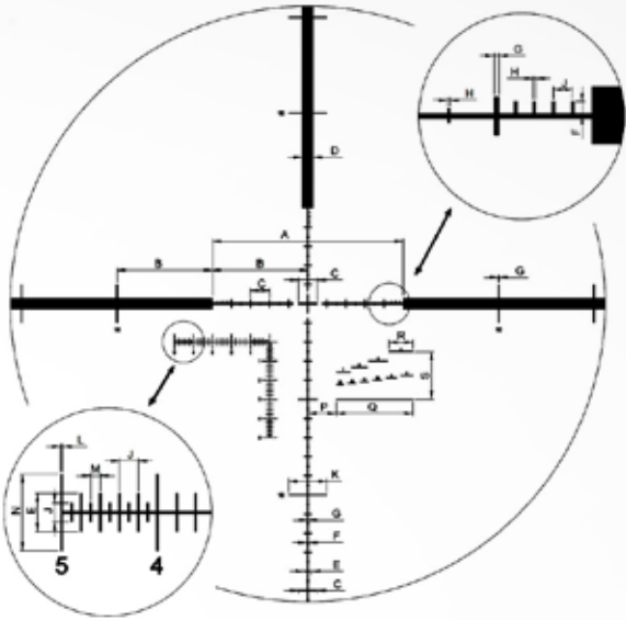
MSR RETICLE RETICLE SUBTENSIONS
