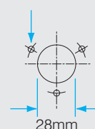
Mounting detail
