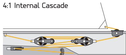
4:1 Internal Cascade
