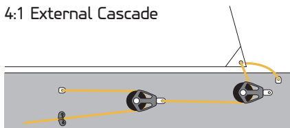
4:1 External Cascade
