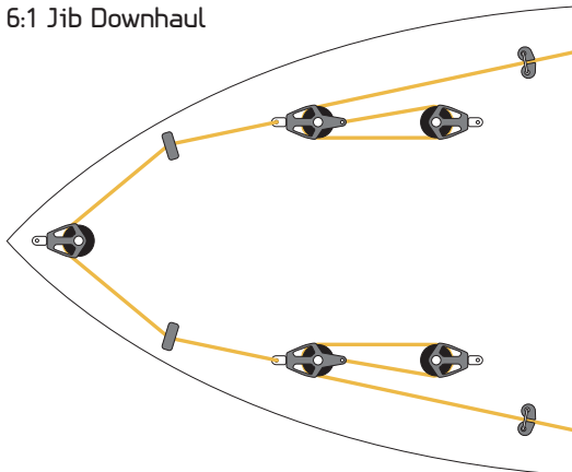
6:1 Jib Downhaul
