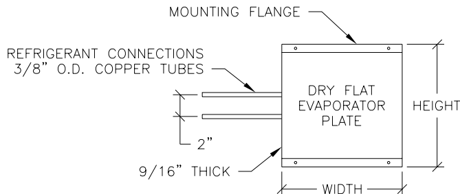
HORIZONTAL PLATE SHOWN SEE FRONT OF THIS SHEET FOR VERTICAL PLATE CONFIGURATION
