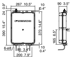
Antennenkoppler AT-1560-15/25
