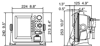
7" LCD (Bügelmontage)
