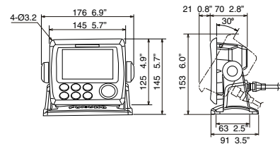
RD-33 Display (Bügel-Montage) 0.9 kg 2.0 lb
