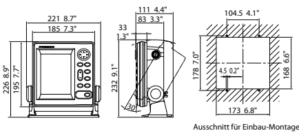
LS-6100 Display 1.3 kg 2.9 lb
