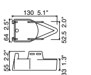
Geber 520-5PWD (Plastik, Heckmontage)
