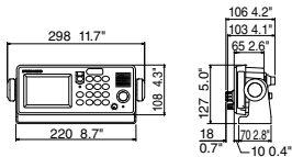
FS-1570/2570
