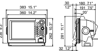
10.4" LCD (Bügelmontage)
