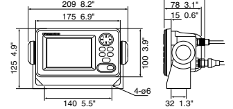
NX-300 Monitor 0.68 kg 1.5 lb
